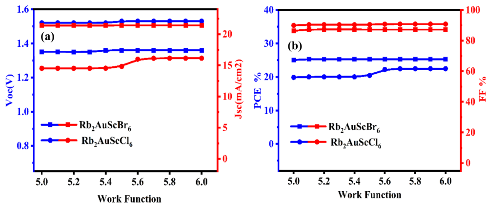
Fig. 8 Effect of Metal Back Contact on performance parameters (a) V_{oc} and J_{sc} , (b) PCE and FF of (ITO/IGZO/ \text{Rb}_2\text{AuScBr}_6 /CBTS/Ni) (ITO/ \text{WS}_2 / \text{Rb}_2\text{AuScCl}_6 /CBTS/Ni) devices.
