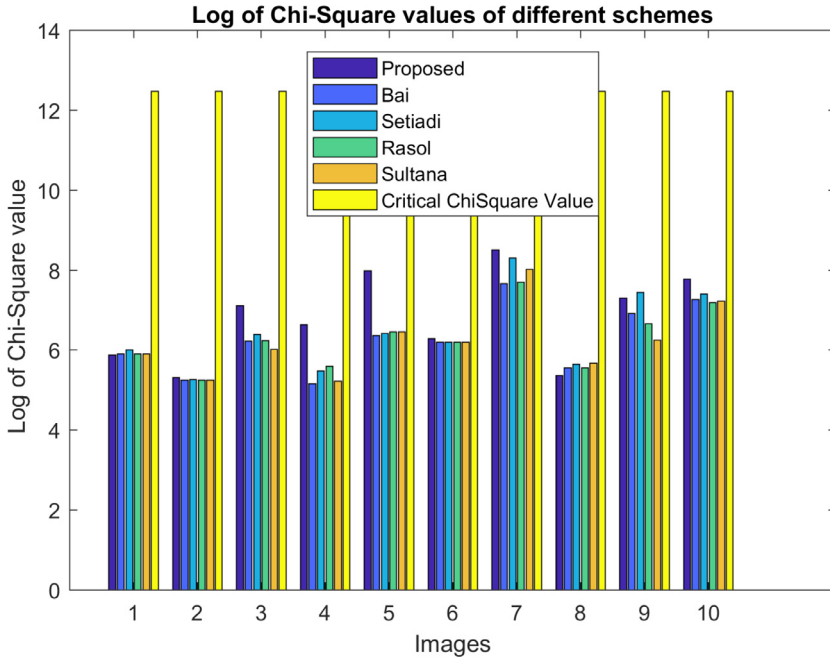
Fig. 16. Comparison of chi-square values among the schemes in the logarithmic scale.
