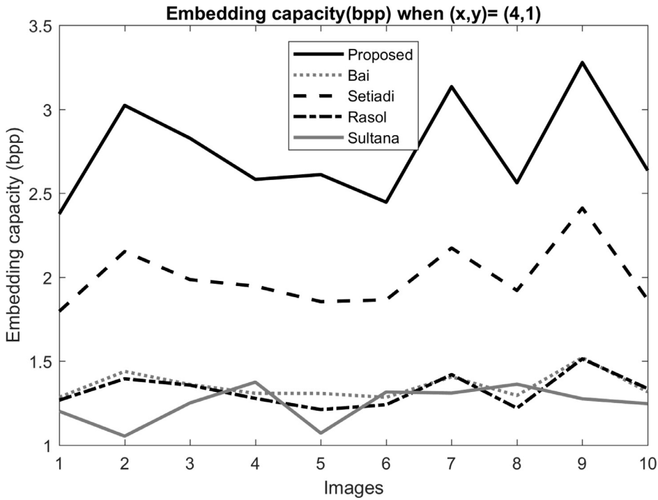
Fig. 7. Comparison of embedding rate. This figure is generated by embedding at (x,y)=(4,1) . The figure states that the proposed scheme yields embedding capacity at a dominating rate which is about 50% higher than Setiadi, 70% higher than Rasol et al., 80% higher than Bai et al. and 90% higher than Sultana et al.
