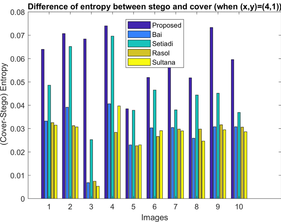
Fig. 12. Difference of entropy between cover and stego. The differences are very small and insignificant to mention.
