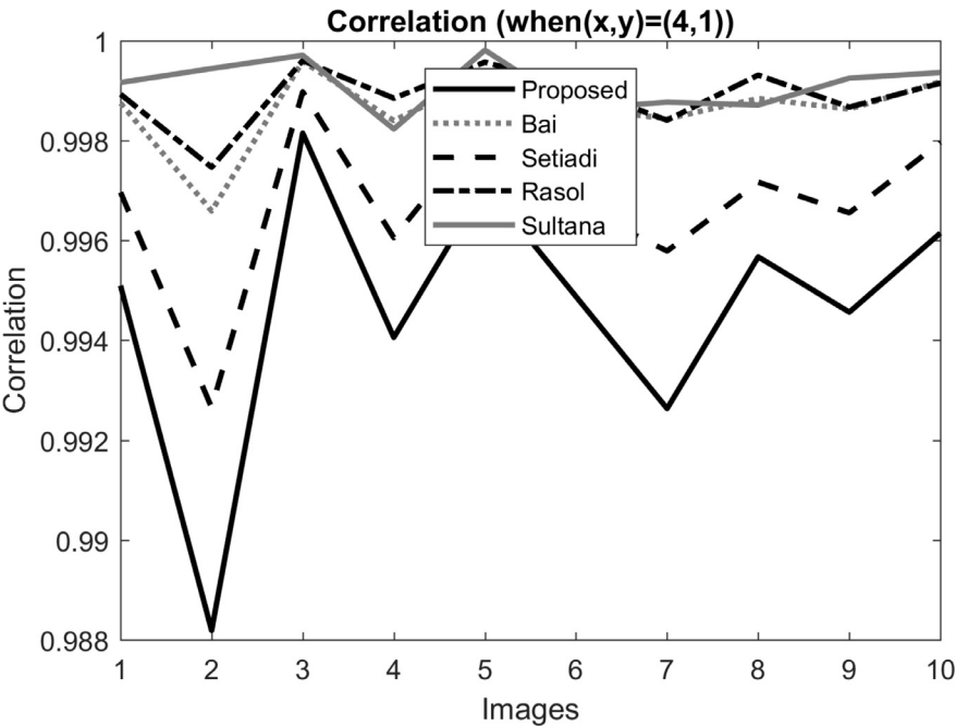
Fig. 11. Correlation coefficients. All the schemes present higher correlations.
