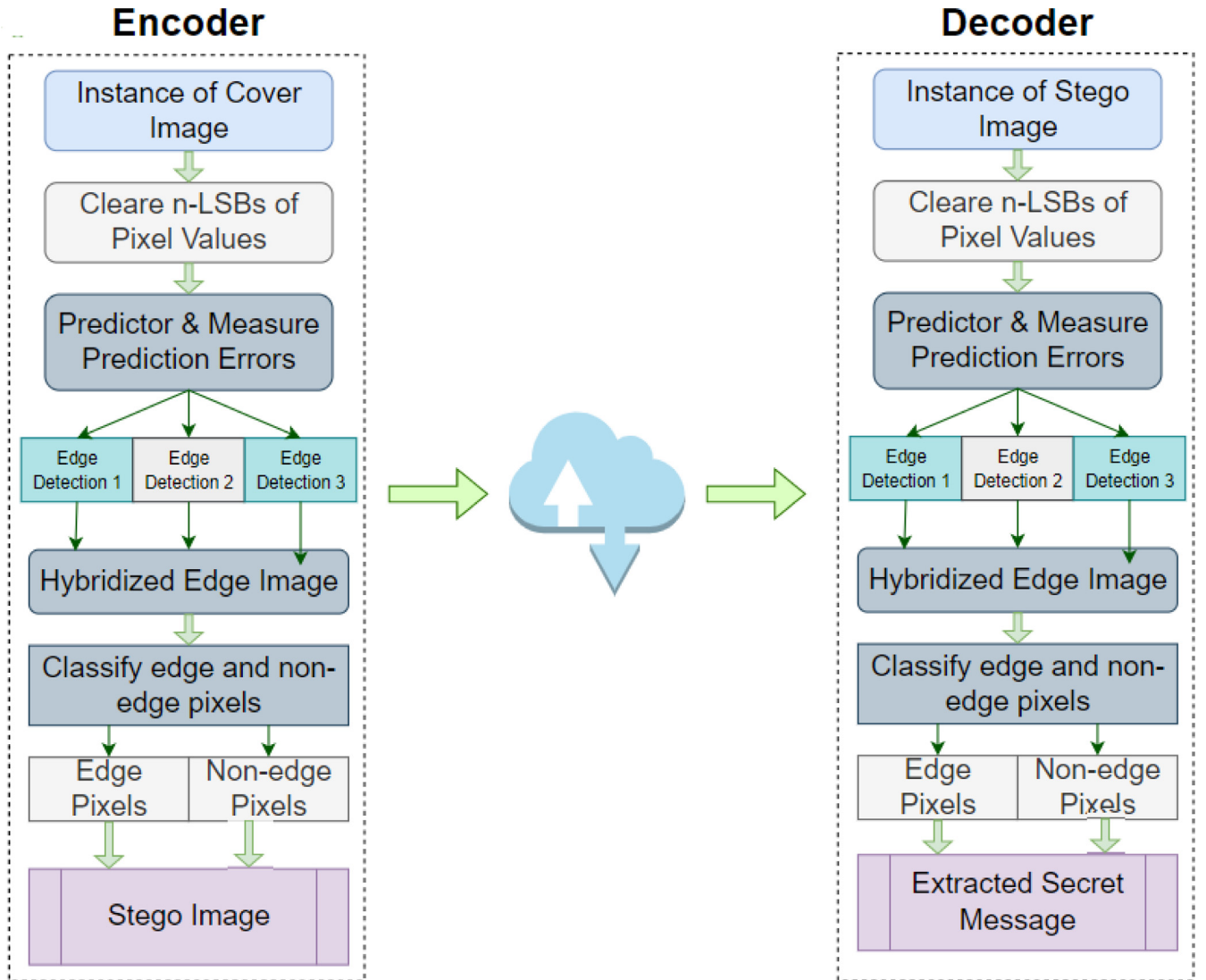
Fig. 1. The Encoder-Decoder architectures of the Proposed Method.
