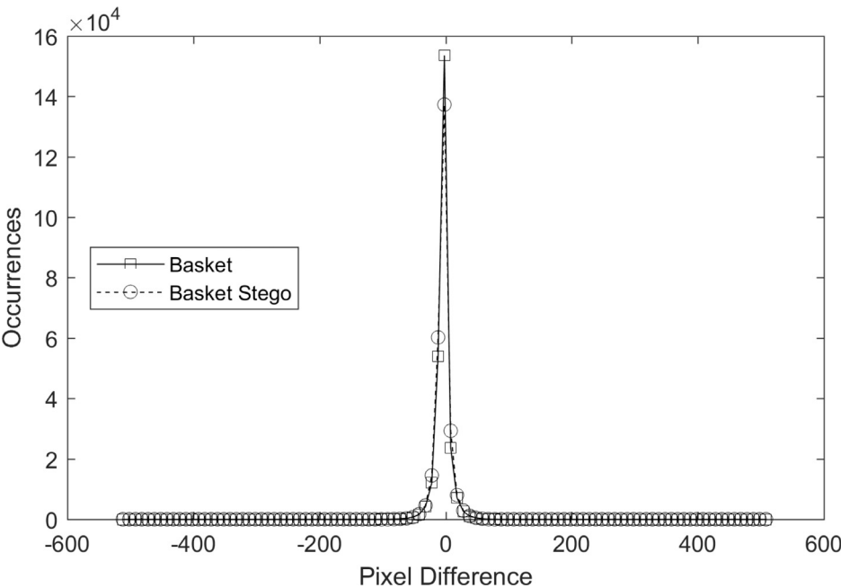
Fig. 15. Pixel Difference Histogram of Basket.
