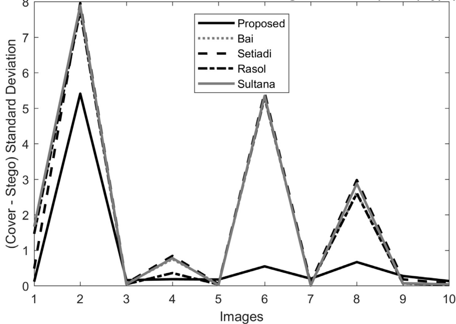
Difference of standard Deviation between stego and cover (when(x,y)=(4,1))
