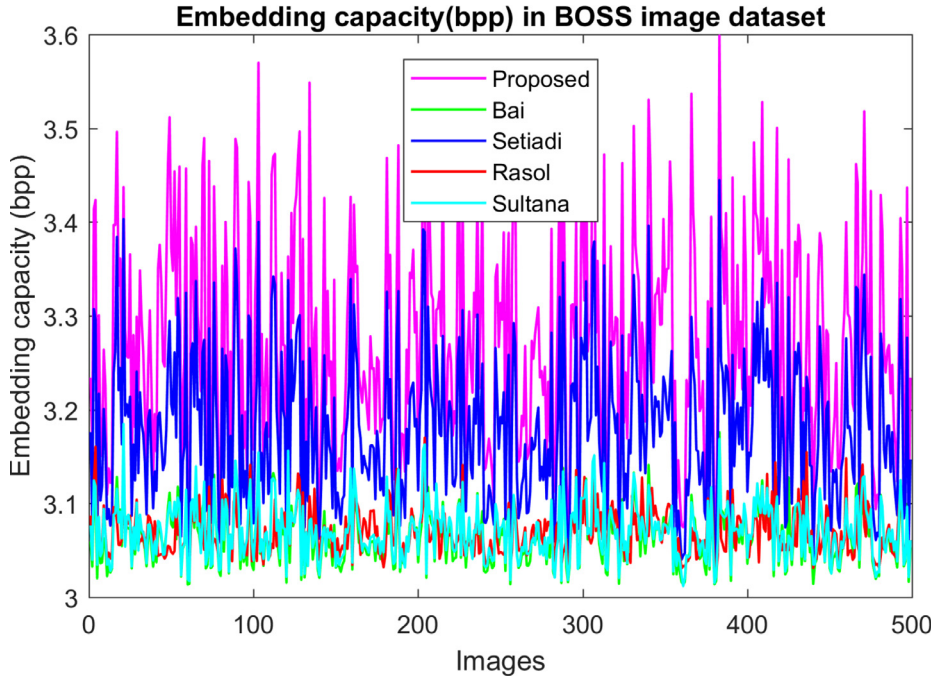
Fig. 8. Performance comparison of the proposed scheme with Bai, Setiadi, Sultana, and Rasol in terms of capacity in the BOSS image dataset. That experiments were done to justify the proposed scheme in a large image dataset. The figure states that our proposal is unbeaten in producing a larger embedding capacity.
