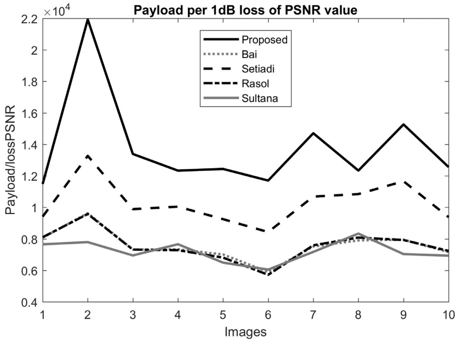
Fig. 9. Number of embedded bits per 1dB loss of PSNR. Regarding that per 1dB loss of PSNR, the proposed scheme noticeably dominates the other competing schemes.
