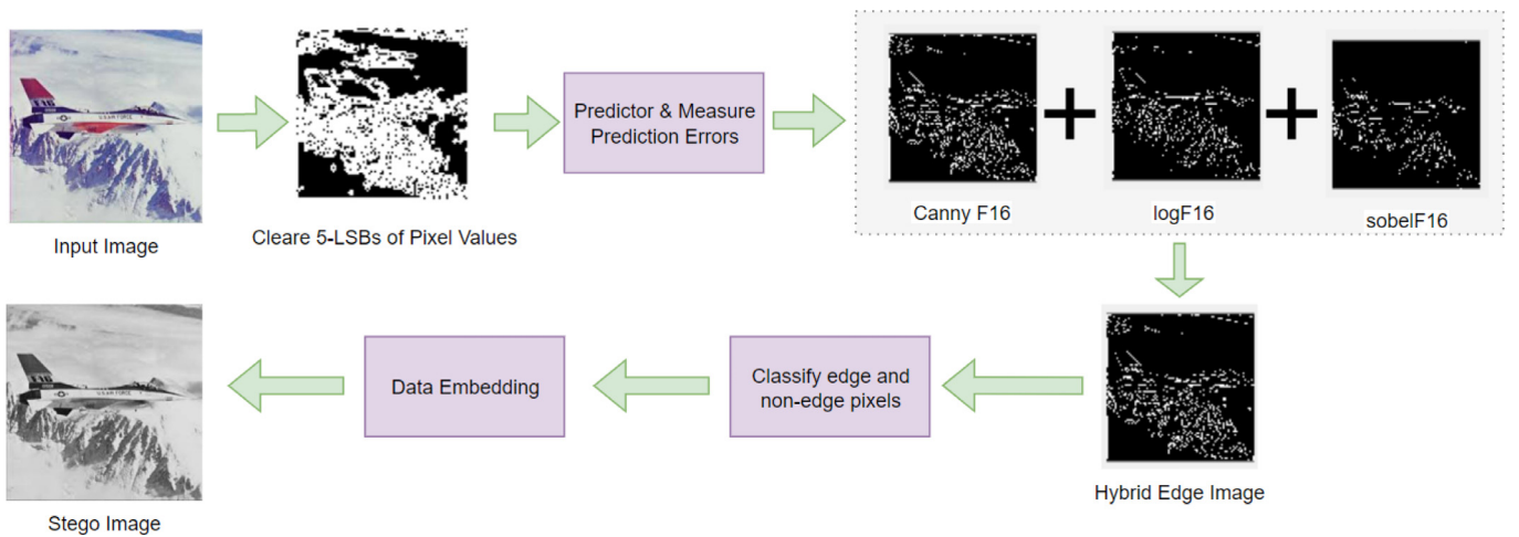
Fig. 2. The top-level overview of the Proposed Method.
