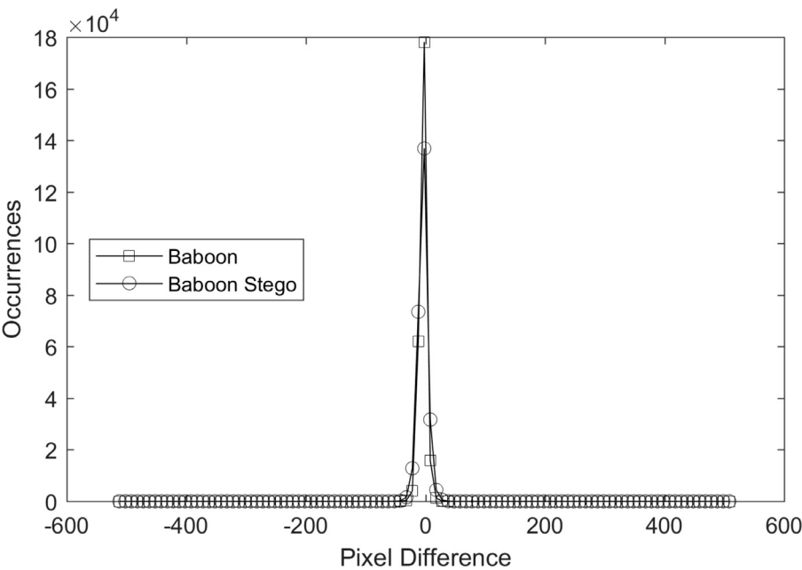
Fig. 14. Pixel Difference Histogram of Baboon.
